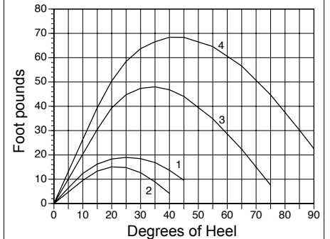
Stability Curves
