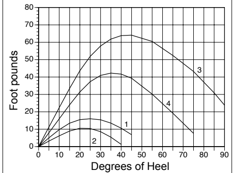
Righting/Heeling Moments (Fixed-weight)
