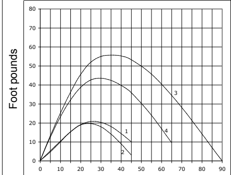
Stability Curves
