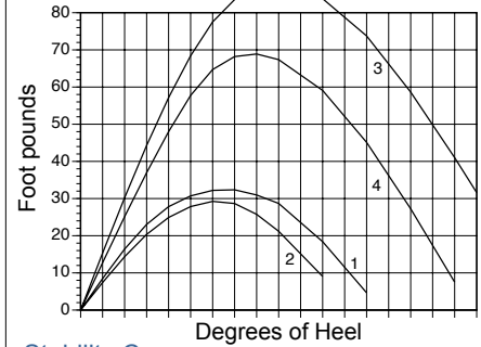
Stability Curves
